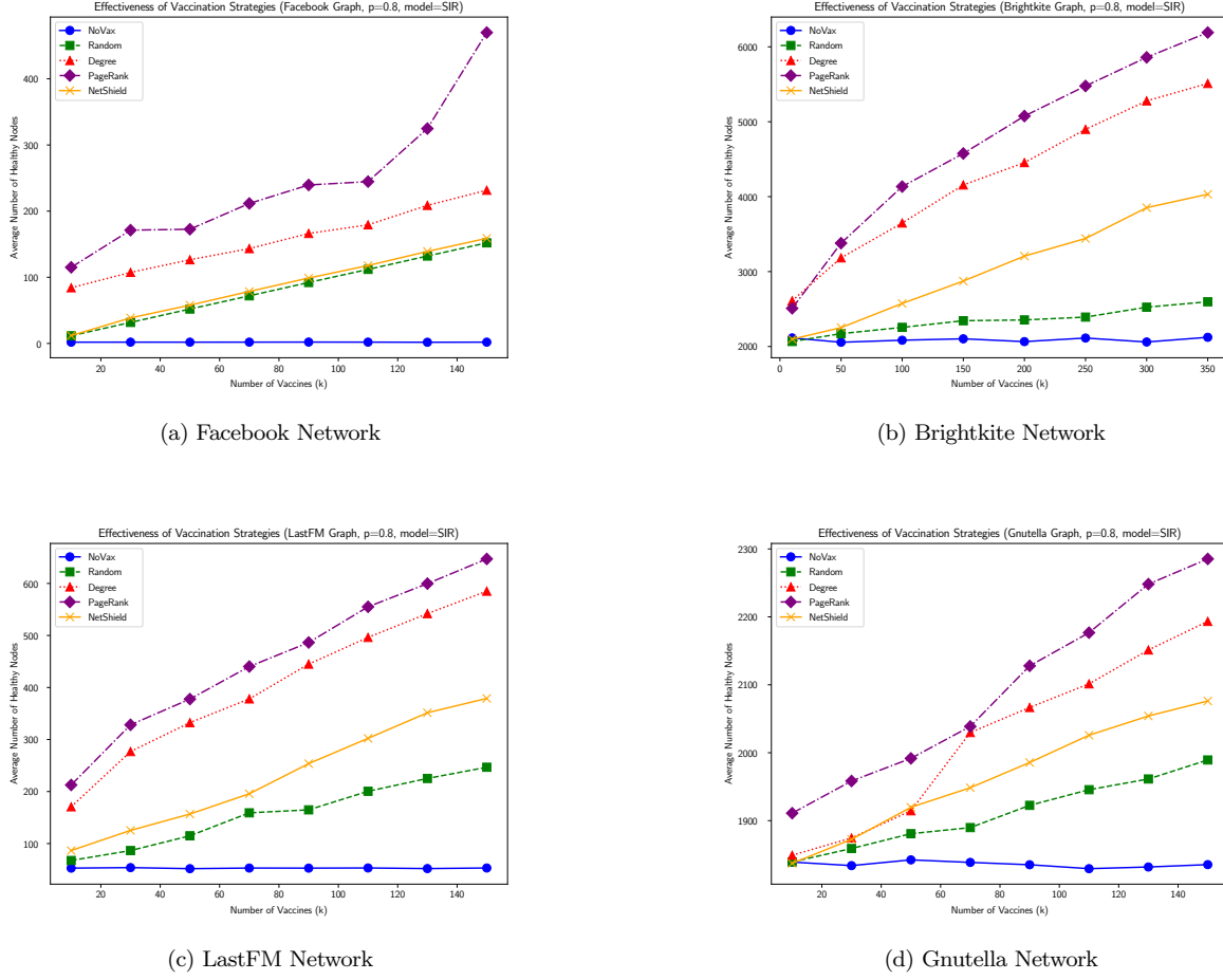
Figure 2: Effectiveness of Vaccination Strategies under the SIR Model ( p=0.8 , \delta=0.1 )
